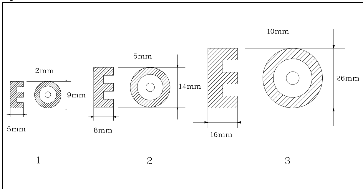
Figure 4. Detection distance
